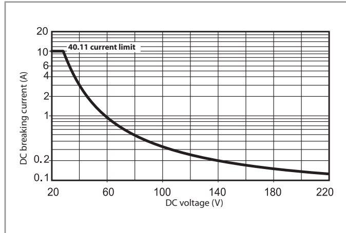
H 40.2 - Maximum DC1 breaking capacity Type 40.11
