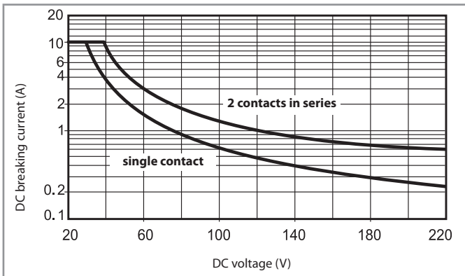
H 40.6 - Maximum DC1 breaking capacity Type 40.62
