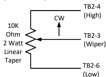
Figure 4 – Potentiometer
