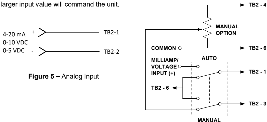
Figure 6 – Auto / Manual Switch
