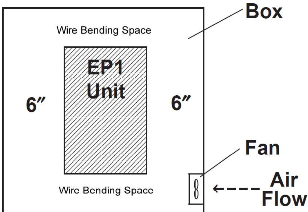
Figure 1 - Enclosure
